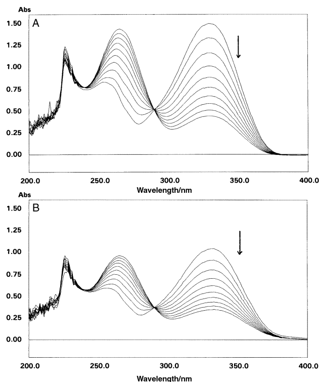
Fig. 1 Decomposition (absorbance values versus wavelength in nm) of imidazotetrazines in phosphate buffer at pH 7.4: A, temozolomide ( 1b ); B, the bis(imidazotetrazine) ( 16c ). Spectra were recorded at intervals of 15 min for A; 30 min for B.
