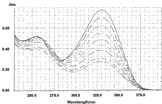
Fig. 2 Decomposition (absorbance values versus wavelength in nm) of bis(imidazotetrazine) 16l in phosphate buffer at pH 7.4. Spectra were recorded at intervals of 5 min.
