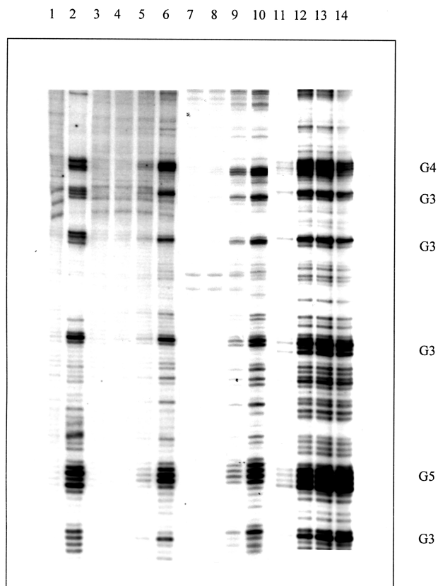
Fig. 3 Partial autoradiogram of 6% denaturing sequencing gel showing the blocks to Taq DNA polymerase after treatment with agents: lane 1, control of unmodified Bam HI- Sal I fragment of pBR322 DNA; lane 2, cisplatin at 1 \mu M; lanes 3–6, mitozolomide ( 1a ) at 1, 10, 100 \mu M and 1 mM, respectively; lanes 7–10, temozolomide ( 1b ) at 1, 10, 100 \mu M and 1 mM, respectively; lanes 11–14, the bis(imidazotetrazine) 16l at 30, 100, 300 \mu M and 1 mM, respectively. Bands marked G3–G5 refer to sequences of 3–5 consecutive guanine residues.
